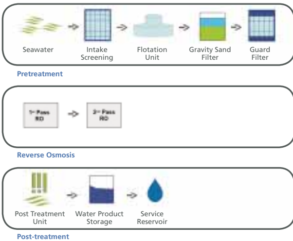
(Top) SingSpring is the largest reverse osmosis seawater desalination plant in Asia.
